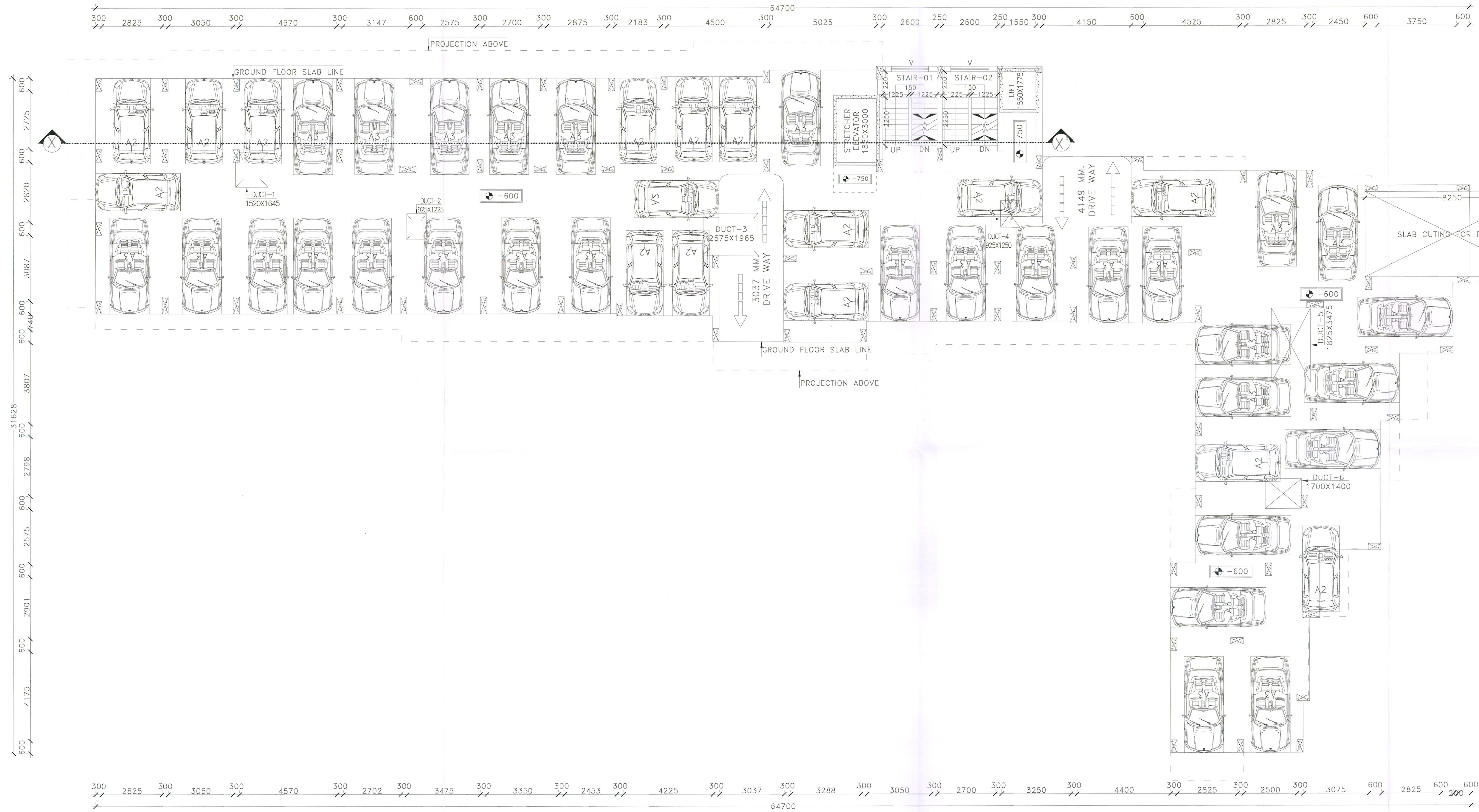
G GROUND FLOOR PLAN SCALE: 1:100
